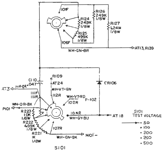
Figure 7-3. Type 1863 switching diagram.
