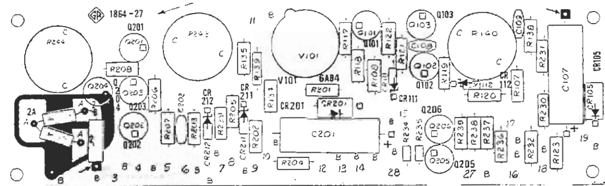
Figure 7-4. Regulator and amplifier circuits etched-board assembly for 1863 and 1864.
