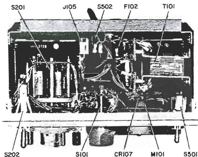
Figure 6-3. Bottom interior view of 1863 Megohmmeter.
