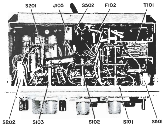
Figure 6-5. Bottom interior view of 1864 Megohmmeter.
